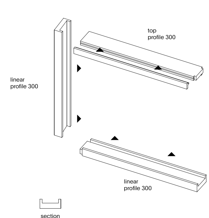
ANCHORING PROFILES
